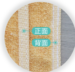
双针链式线迹 Double-needle chain stitches
